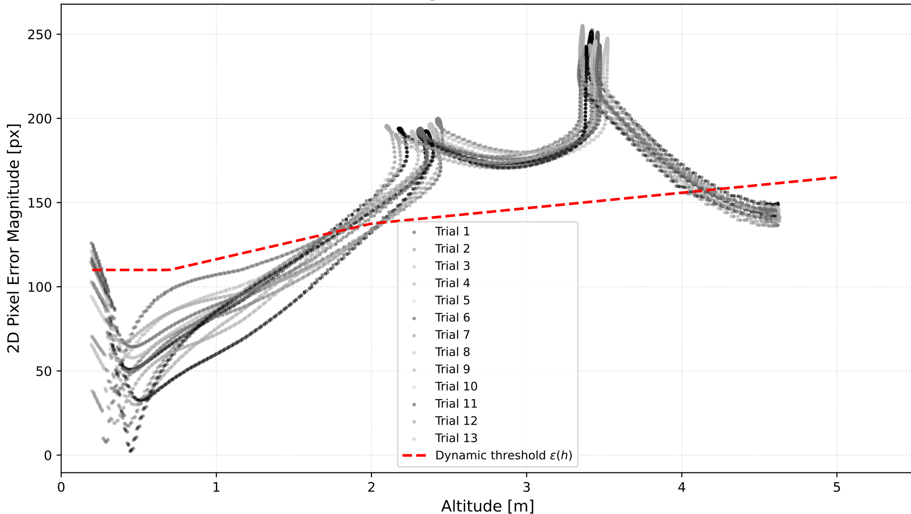
Tracking Error vs. Altitude
